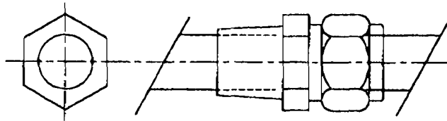
BRASS SWAGELOK MALE CONNECTOR PART NO. B-810-1-6
